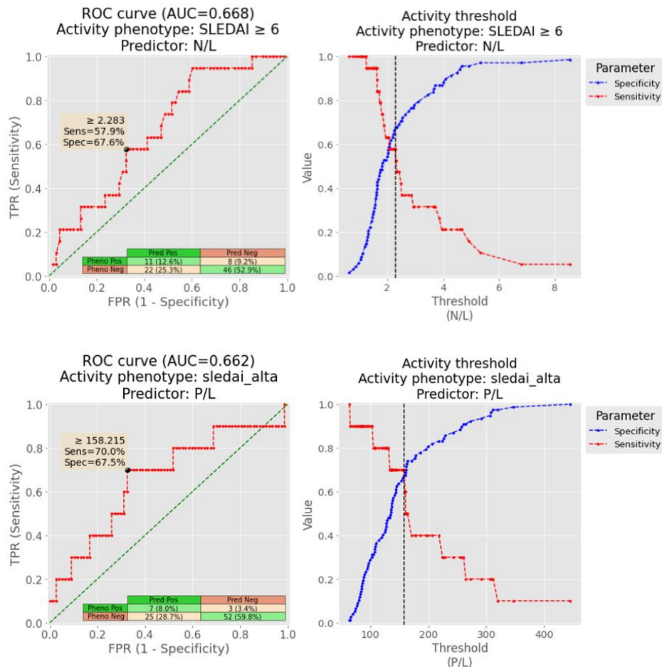
FIGURE 3. ROC CURVE FOR NLR, PLR AND SLEDAI ( \geq 6 ). (N=87)
